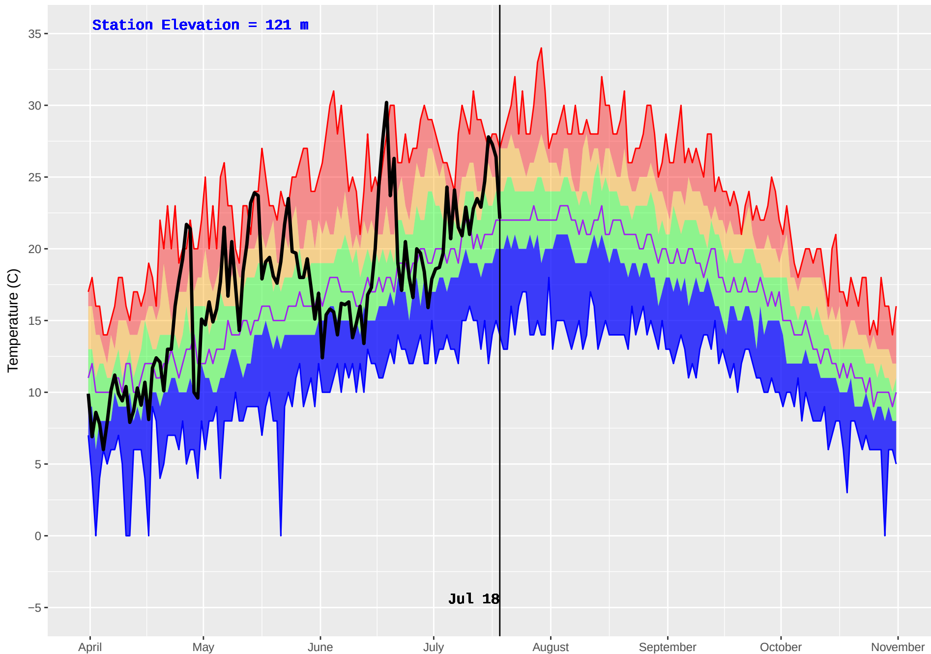
BOWSER (56) : Historical (1985–2016) and Current (2018) Daily Temperature
