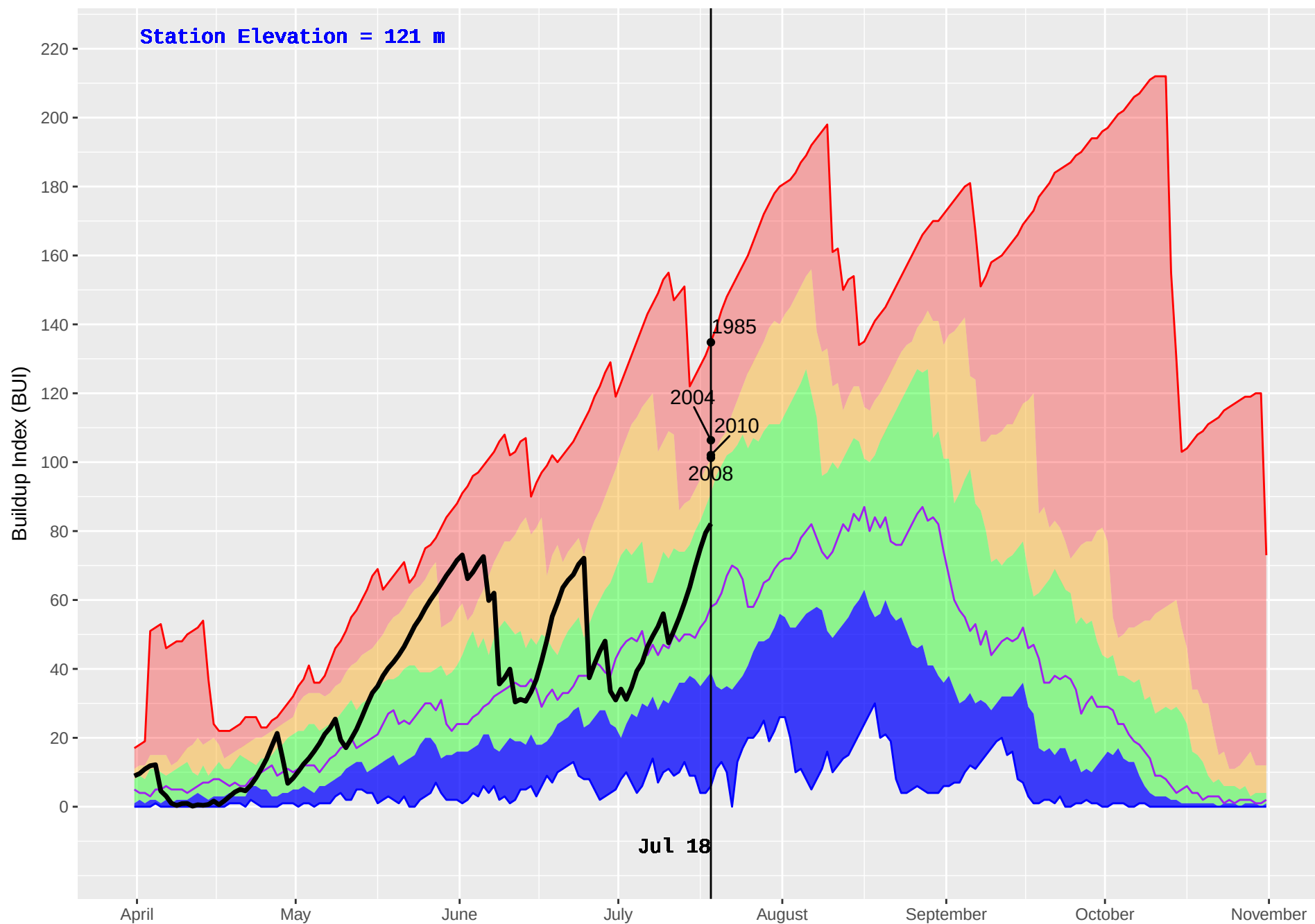
BOWSER (56) : Historical (1985–2016) and Current (2018) Daily Buildup Index (BUI)
